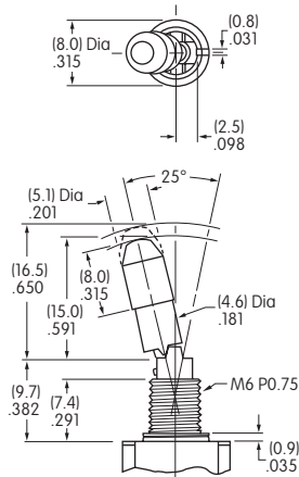
LL4 6mm/.291" (7.4mm) 螺纹型有键槽
