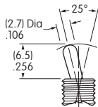
S3 .256" (6.5mm) 搬动杆
